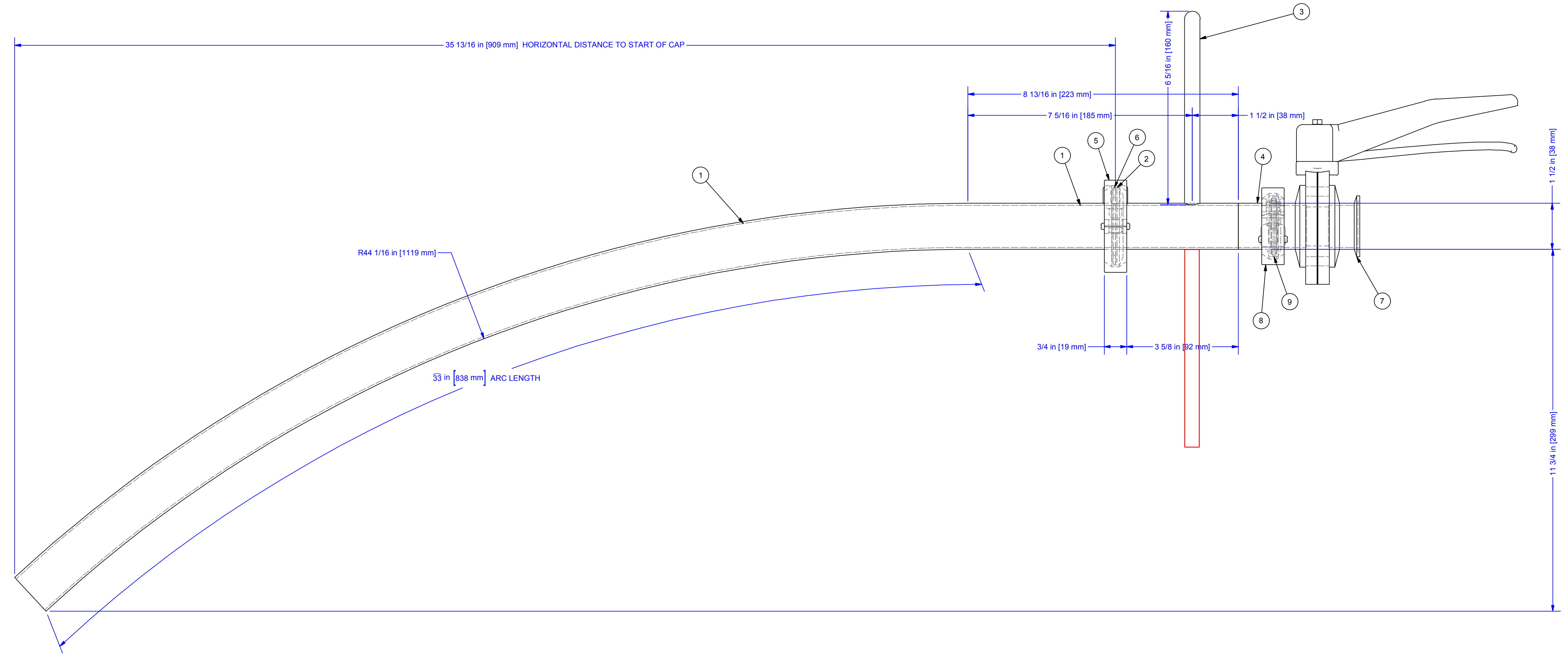
RACKING ARM ASSEMBLY SCALE 1/2
