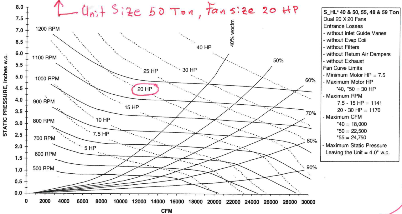
Figure 50. 40 & 50, 55 / 48 & 59 Ton supply fan performance without Inlet Guide Vanes (IGV)
